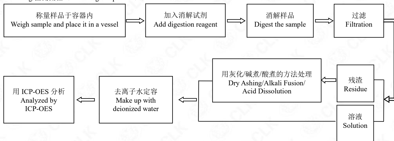
Pb/Cd/Hg 检测流程 (Pb/Cd/Hg test process) :
